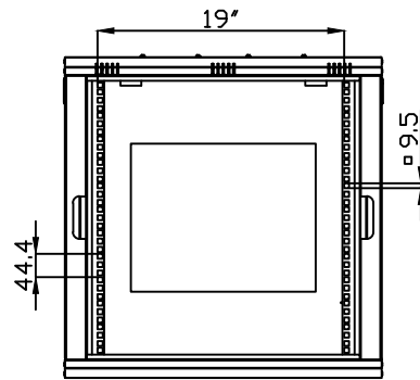
Front View Without the Door
