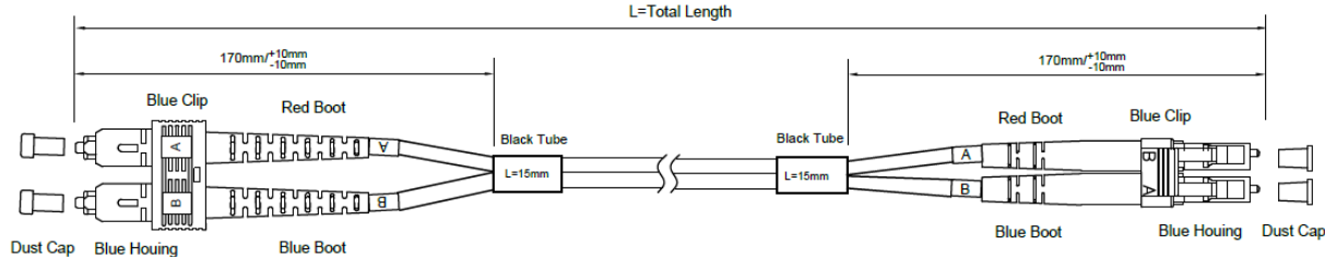
Example SM OS2 - SC to LC
